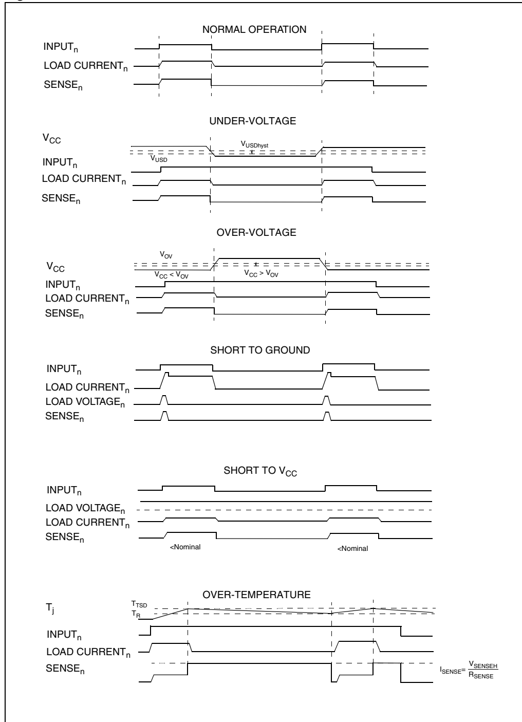
Figure 6. Waveforms
