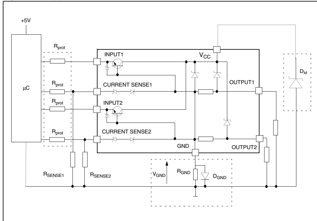
Figure 19. Application schematic
