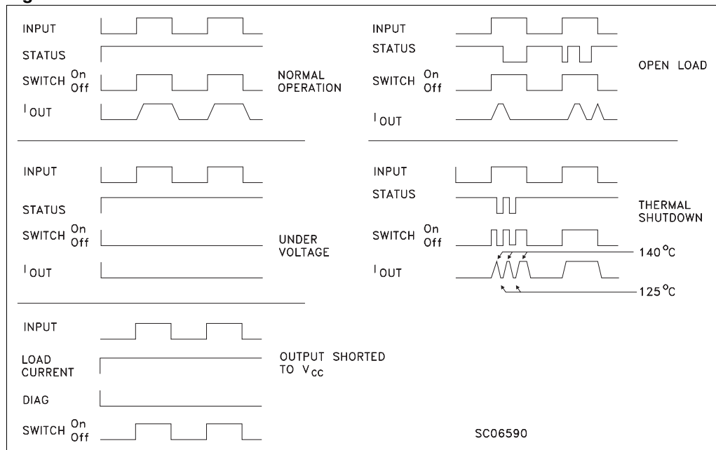
Figure 7. Waveforms
