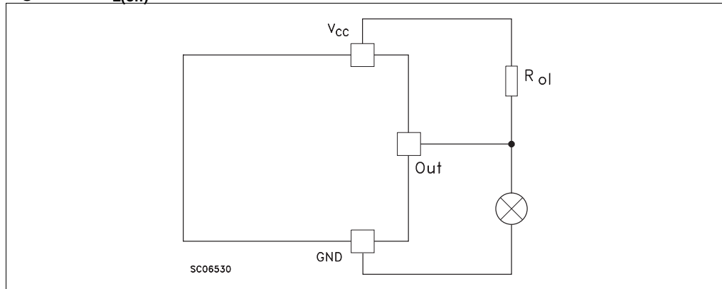
Figure 4. I_{L(off)} circuit
