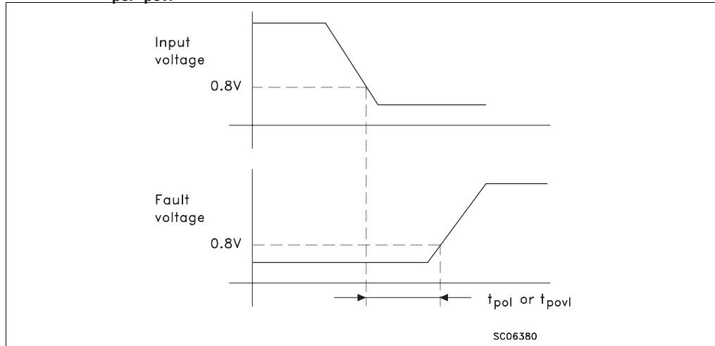
Figure 5. t_{pol}/t_{povl} waveforms
