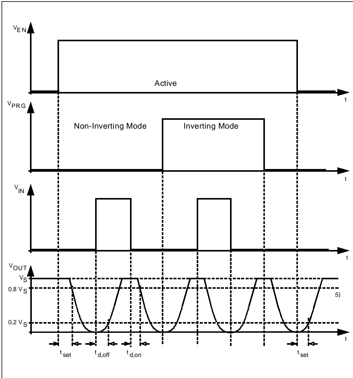
Figure 1. Timing Characteristics
