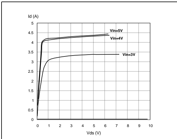
Figure 25. Output characteristics
