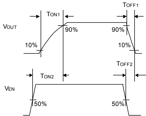
Fig.3 Timing diagram
