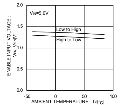
Fig.9 EN, /EN input voltage
