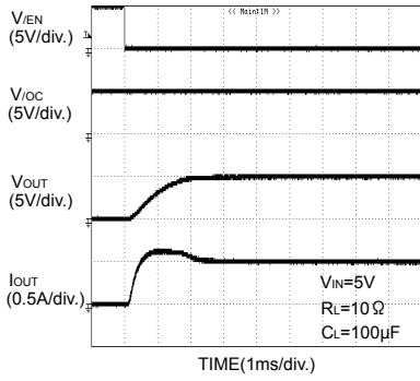
Fig.28 Output rise characteristic (BD2061AFJ)
