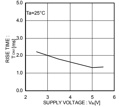
Fig.18 Output rise time
