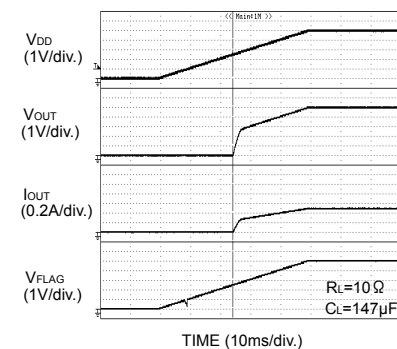
Fig.68 UVLO V IN increasing (BD6519FJ)
