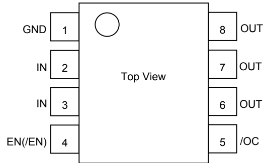
Fig.71 Pin Configuration
