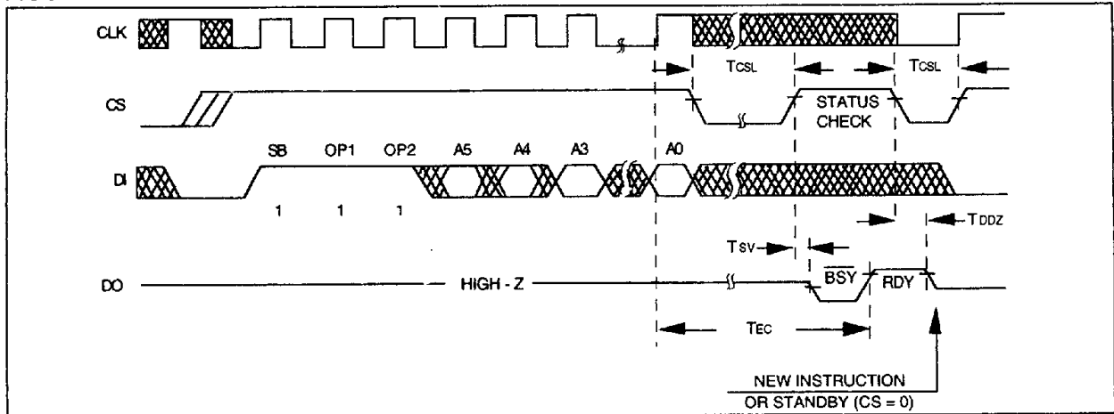
FIGURE 2-4: ERASE/WRITE ENABLE/DISABLE
