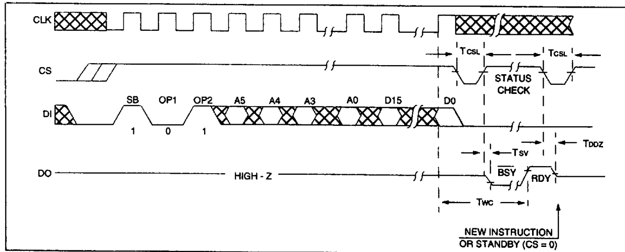
FIGURE 2-2: WRITE MODE
