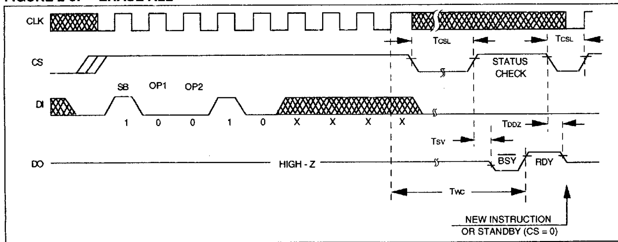
FIGURE 2-5: ERASE ALL
