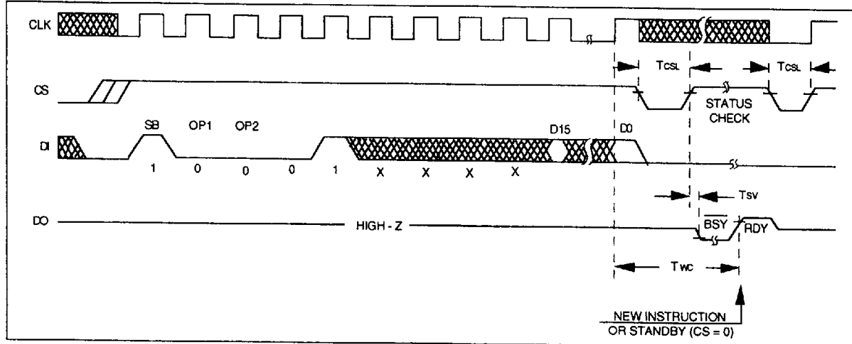
FIGURE 2-6: WRITE ALL
