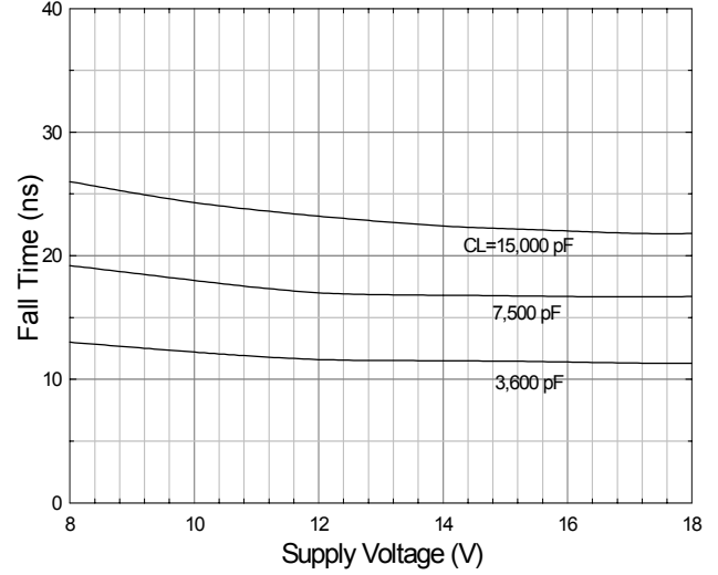
Fig. 5 Fall Time vs. Supply Voltage
