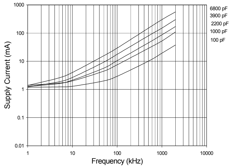
Fig. 18 Supply Current vs. Frequency V cc = 35V
