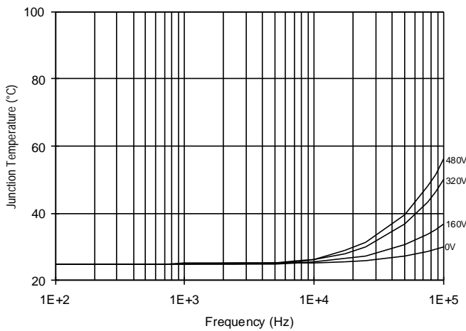
Figure 52. IR2132 T J vs. Frequency (IRF840) R GATE = 15Ω, V CC = 15V
