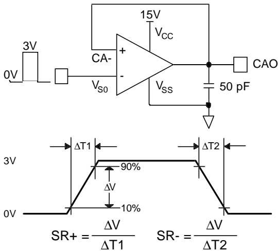
Figure 7. Operational Amplifier Slew Rate Measurement
