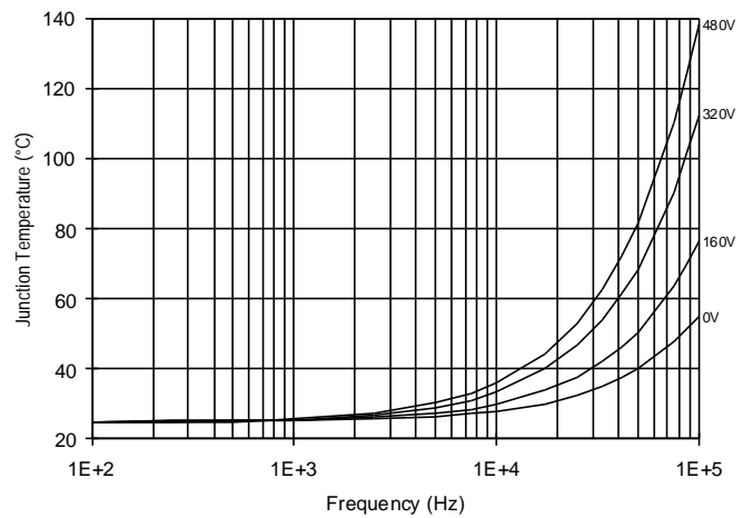
Figure 53. IR2132 T J vs. Frequency (IRF450) R GATE = 10Ω, V CC = 15V
