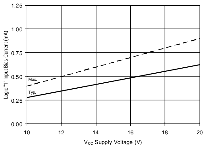
Figure 29A. Logic "1" Input Current vs. Voltage
