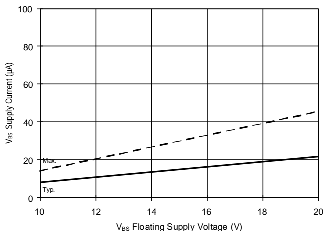
Figure 27B. V BS Supply Current vs. Voltage
