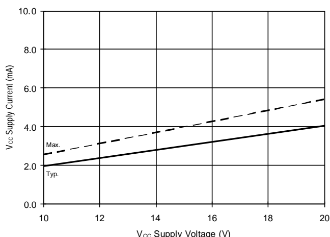
Figure 28B. V CC Supply Current vs. Voltage
