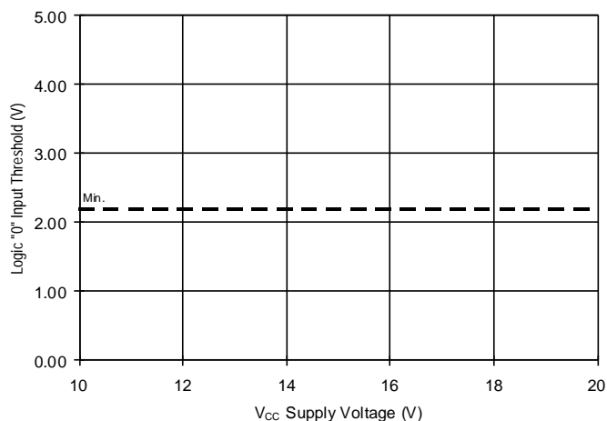
Figure 20B. Logic "0" Input Threshold vs. Voltage
