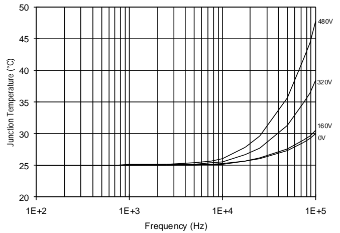
Figure 51. IR2132 T J vs. Frequency (IRF830) R GATE = 20Ω, V CC = 15V
