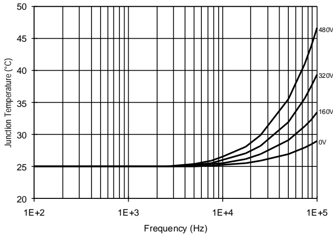
Figure 50. IR2132 T J vs. Frequency (IRF820) R GATE = 33Ω, V CC = 15V
