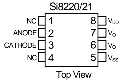
Figure 16. Pin Configuration
