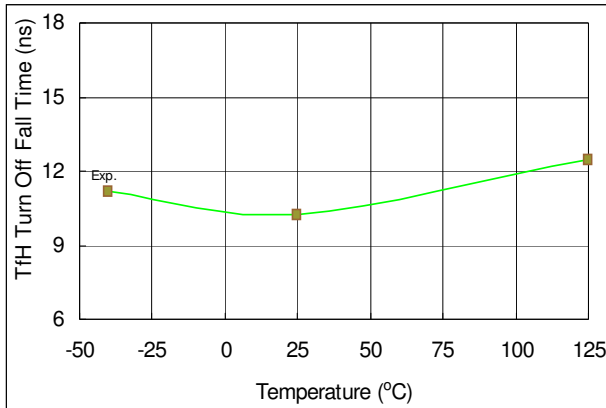
Figure 61. Tfh Turn Off Fall Time vs. Temperature
