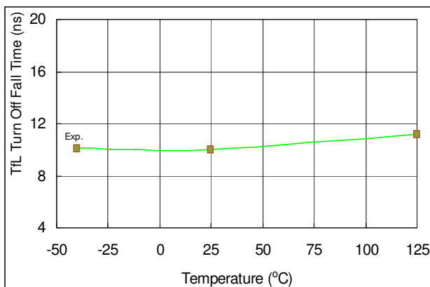
Figure 65. Tfl Turn Off Fall Time vs. Temperature
