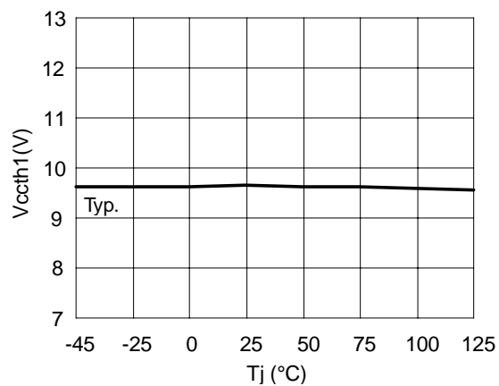
Figure 9. V_{CC} UV Turn On Threshold vs. Temperature
