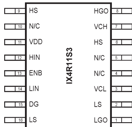
16-PIN SOIC
