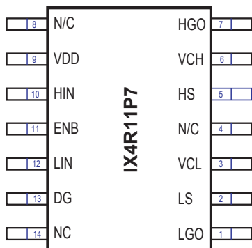
14-PIN DIP
