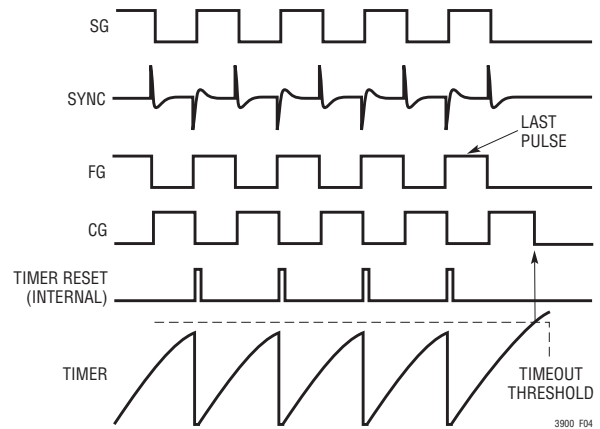
Figure 4. Timer Waveforms
