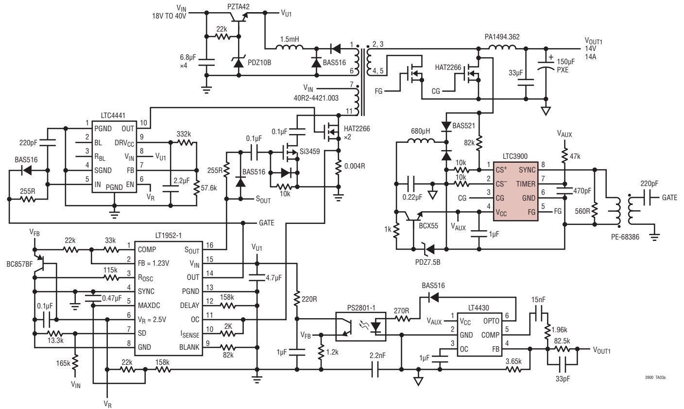
By Using Active Reset and 60V MOSFETs Converter is Achieving 94% to 95% Efficiency with Only Four MOSFETs.
