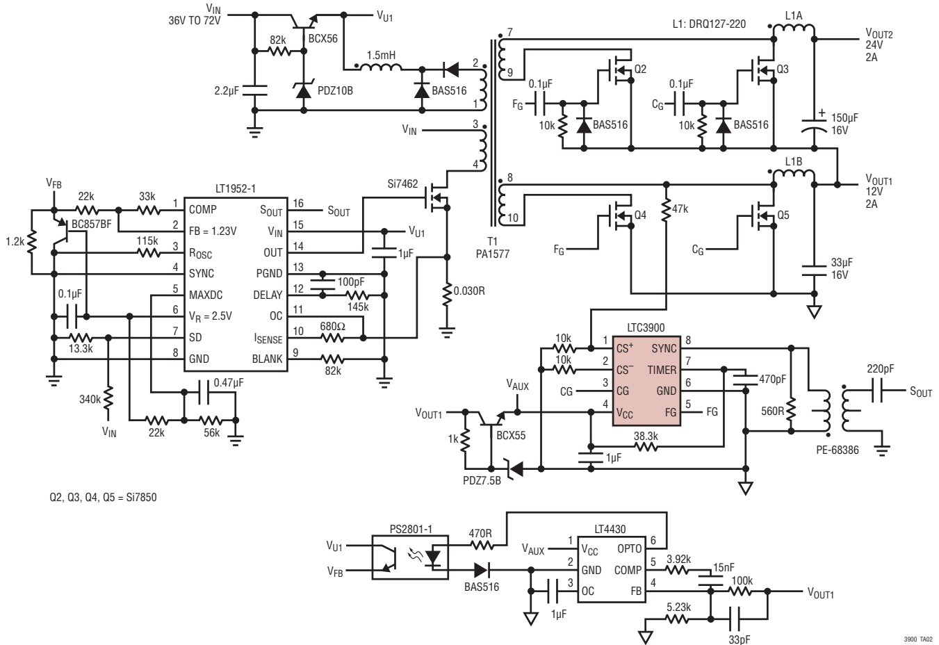
36V to 72V Input to 12V and 24V (or ±12V), 2A Output Converter in 1/8th Brick Footprint
