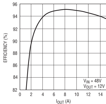
The Efficiency of 12V Output Converter is Over 95% at 8A Output.
