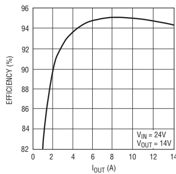
By Using Active Reset and 60V MOSFETs Converter is Achieving 94% to 95% Efficiency with Only Four MOSFETs.
