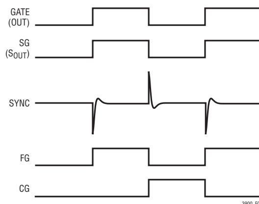
Figure 2. Synchronization Waveforms
