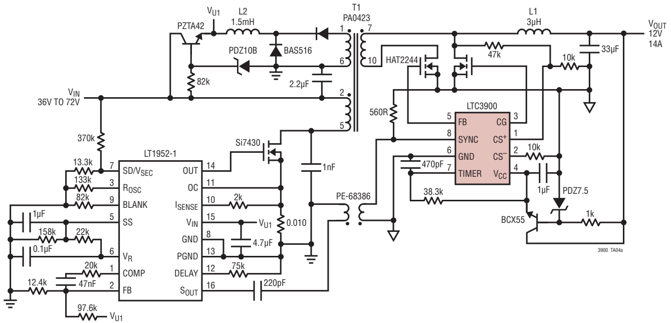
36V to 72V Input to 12V, 14A Output Converter in 1/8th Brick Footprint
