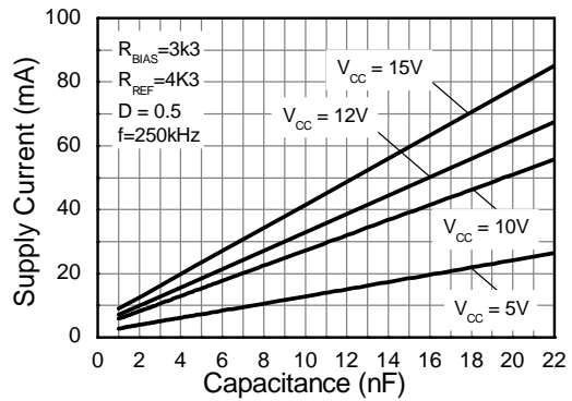
Supply Current vs Capacitive Load
