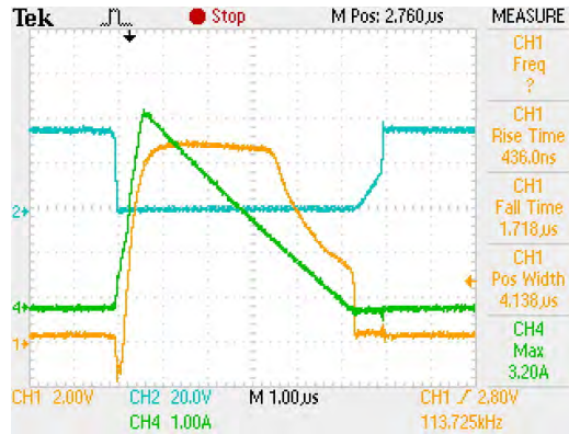
Fig 4a: Critical conduction mode
