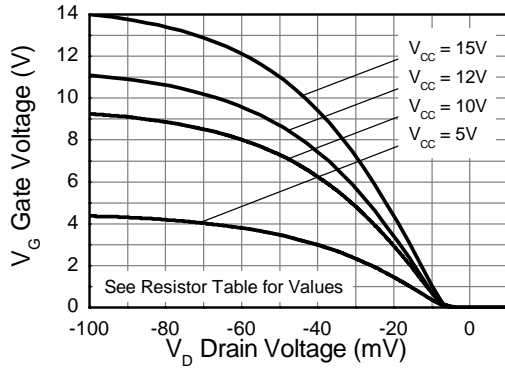
Transfer Characteristic
