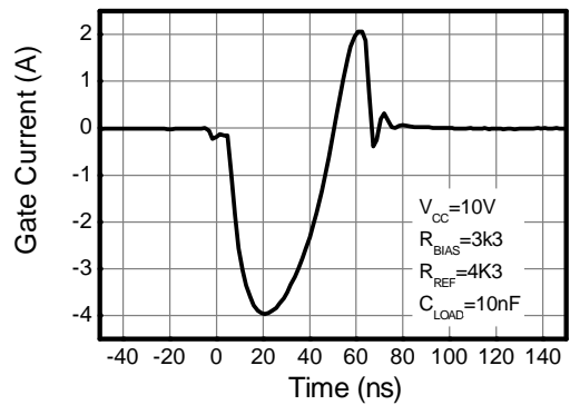
Gate Drive Off Current
