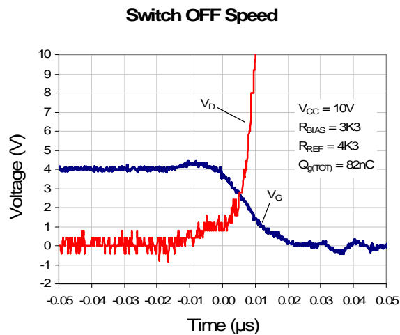
Fig 4c: Typical switch OFF speed when driving a Q_{g(TOT)} = 82\text{nC} MOSFET
