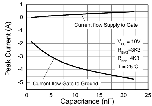
Gate Current vs Capacitive Load
