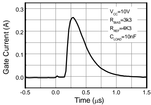
Gate Drive On Current
