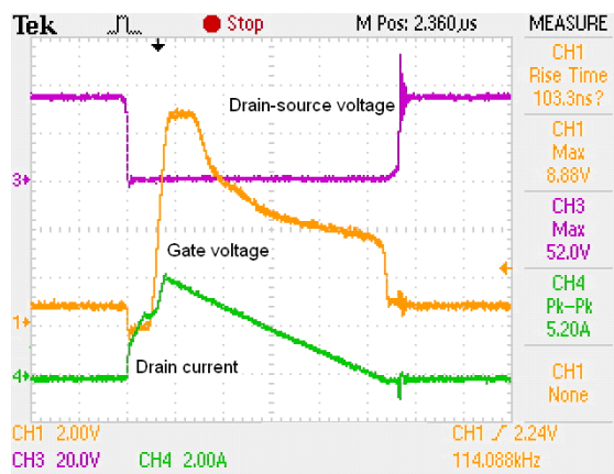
Fig 1b: Critical Conduction Mode (CrCM)
