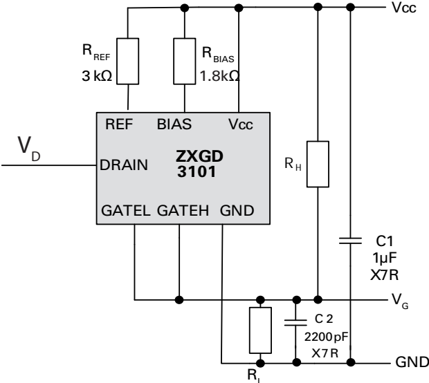
Figure 4: Test circuit
