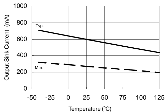
Figure 20A. Output Sink Current vs. Temperature
