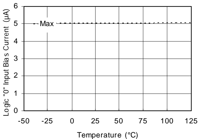
Figure 17A. Logic "0" Input Current vs. Temperature
