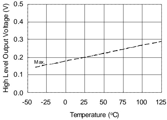
Figure 11A. High Level Output Voltage vs. Temperature (I O = 2 mA)
