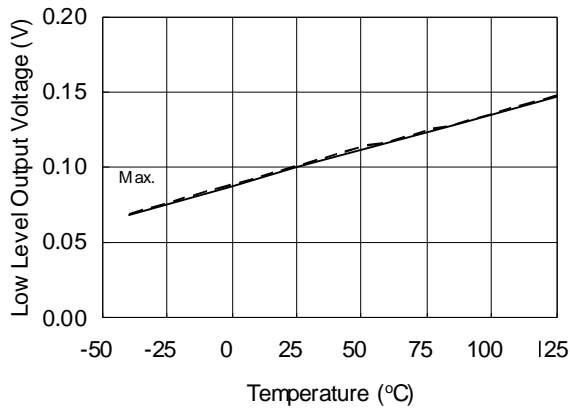
Figure 12A. Low Level Output Voltage vs. Temperature (I O = 2 mA)
