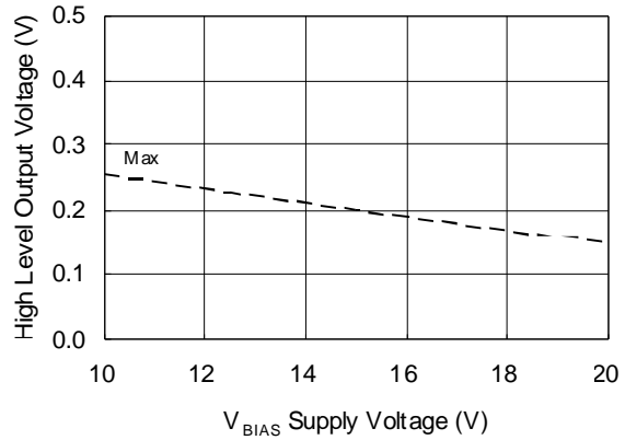
Figure 11B. High Level Output Voltage vs. Supply Voltage (I O = 2 mA)
