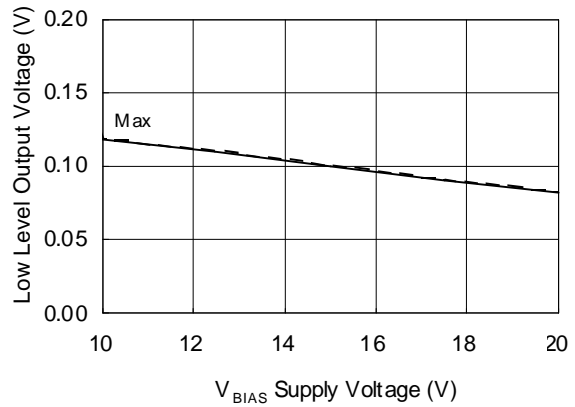
Figure 12B. Low Level Output vs. Supply Voltage (I O = 2 mA)
