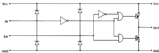
Figure 1B - IXDN409 (Non-Inverting) Diagram
