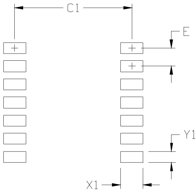
Figure 49. 14-Pin LGA Land Pattern
