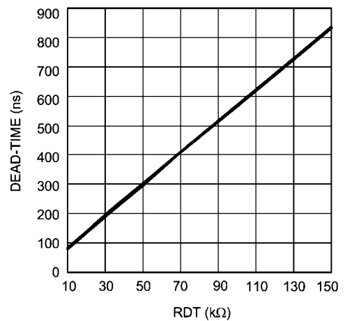
Dead-Time vs RT Resistor Value
