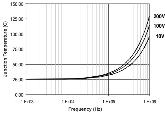
Figure 33. IR2010S Tj vs Frequency R_{GATE} = 16 \text{ Ohm} , V_{cc} = 15V with IRFBC40
