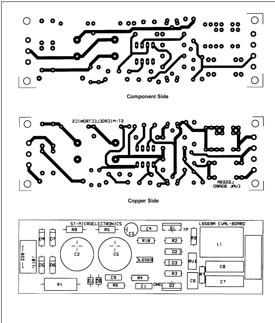
Figure 12. PC Board and Components Layout.
