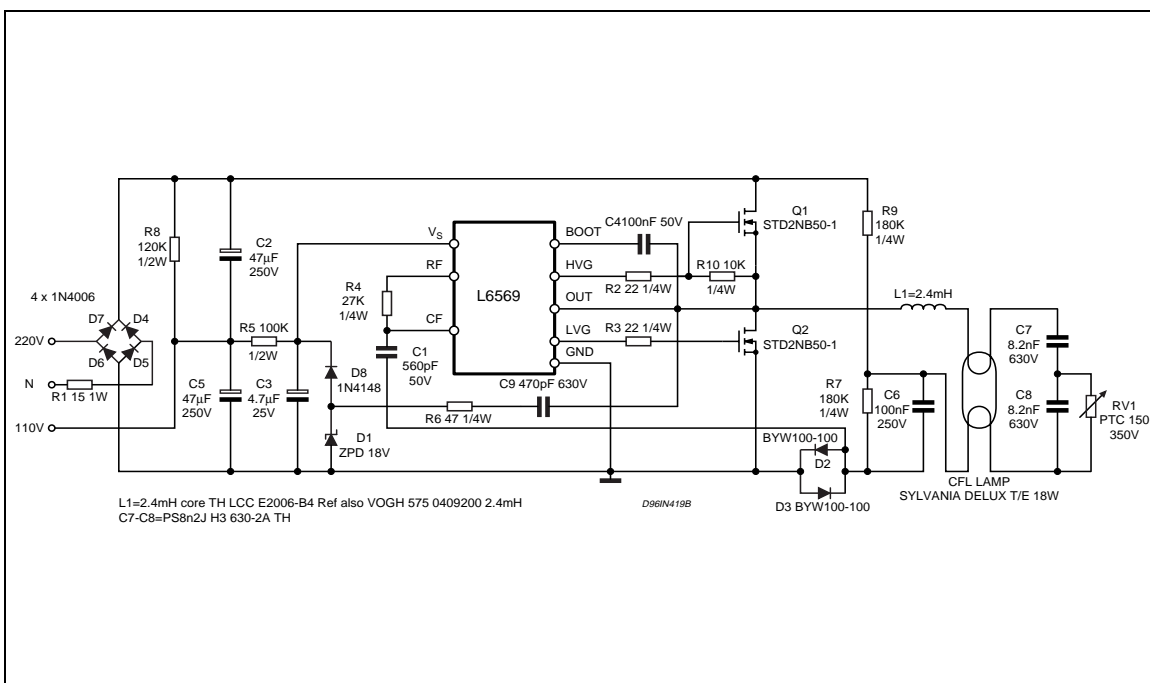
Figure 11. CFL Demoboard 110/220V Inputs.
