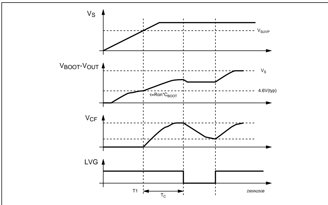
Figure 3. Waveforms (L6569A)
