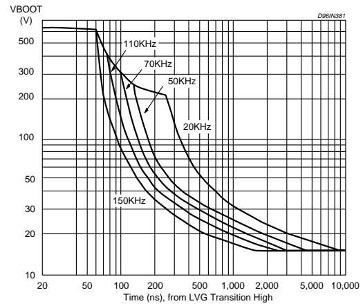
Figure 8. V_{boot} pin SOA @ T_j = 125^\circ\text{C}
