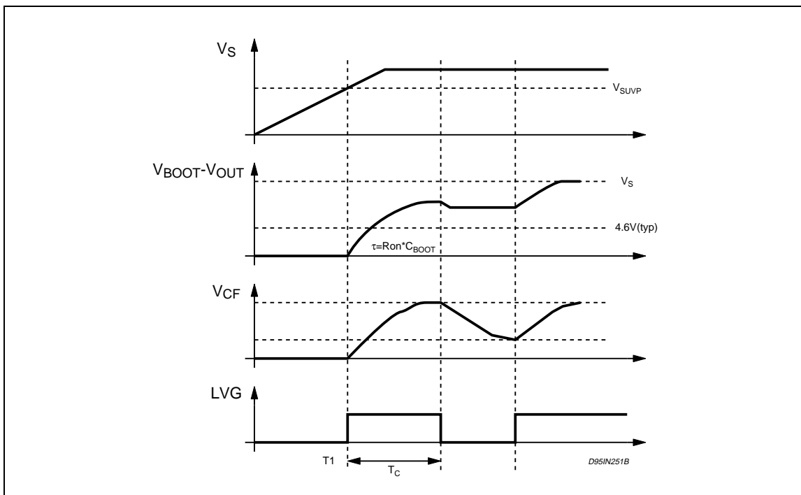
Figure 3. Waveforms (L6569A)
