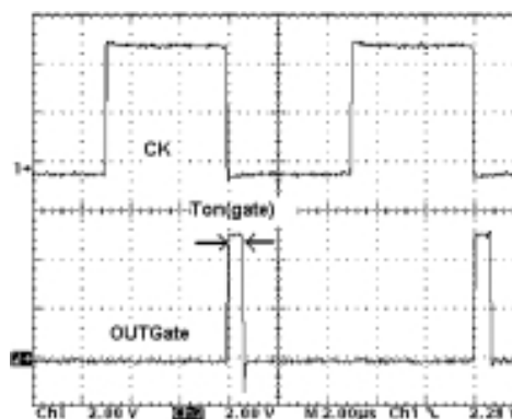
Figure 9 : Minimum T_{ON(GATE)}
