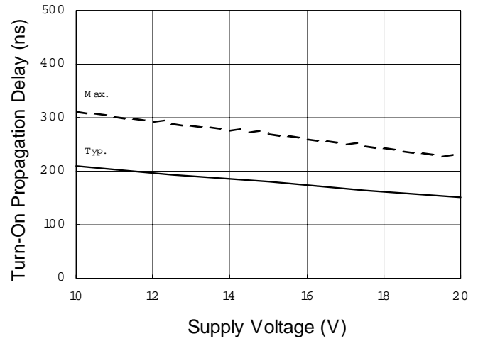
Figure 4B. Turn-On Propagation Delay vs. Supply Voltage
