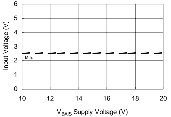
Figure 8B. Logic "1" Input Voltage vs. Supply Voltage
