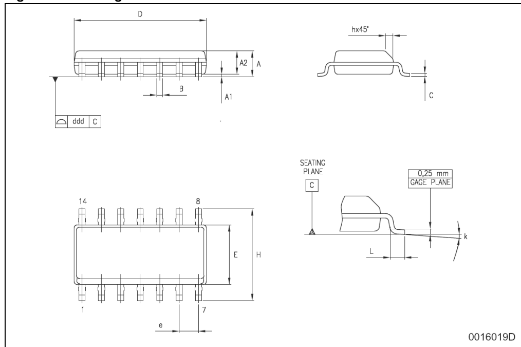
Figure 9. Package dimensions
