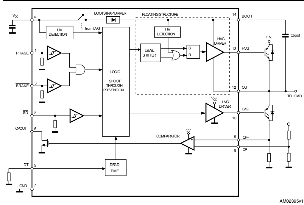
Figure 6. Application diagram
