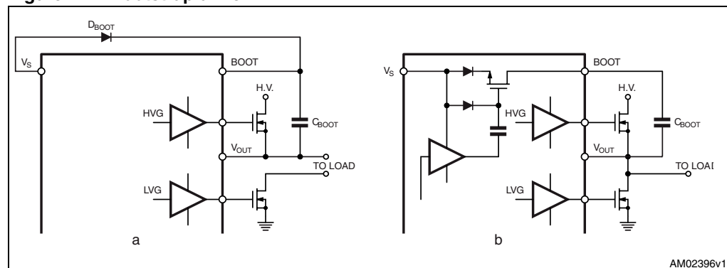
Figure 7. Bootstrap driver
