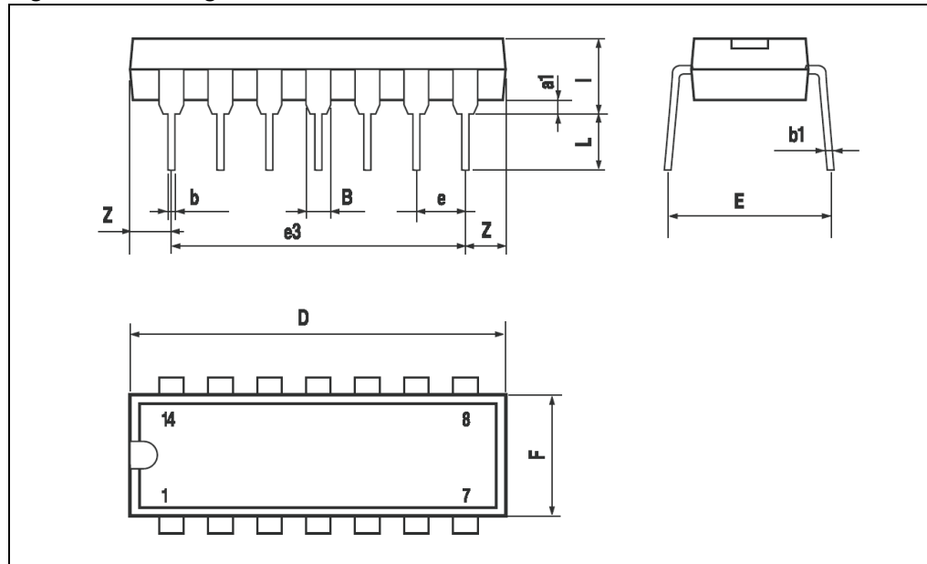
Figure 8. Package dimensions
