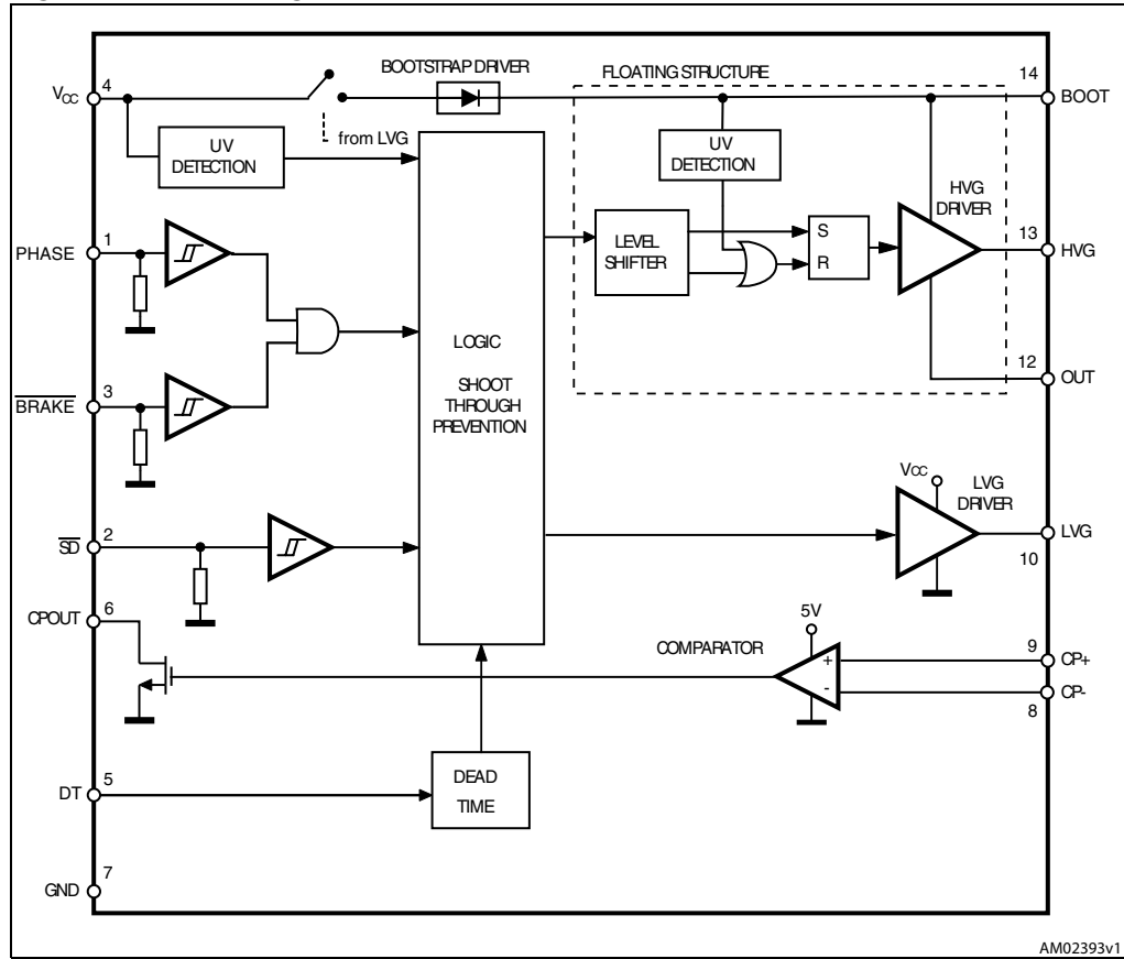
Figure 1. Block diagram
