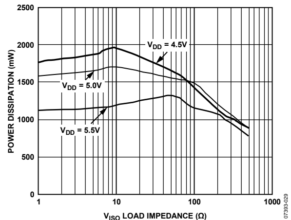
Figure 9. Power Dissipation vs. Load Impedance for Fault Conditions
