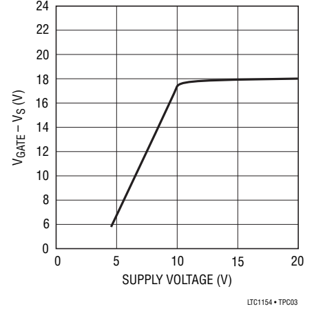
High Side Gate Voltage
