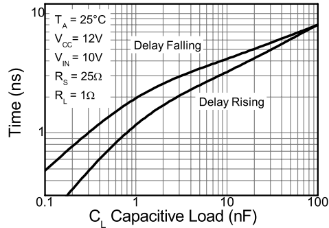
Propagation Delay
