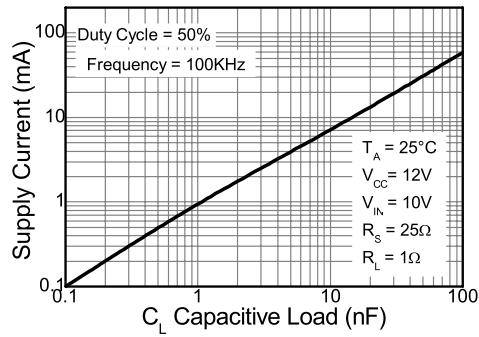
Supply Current
