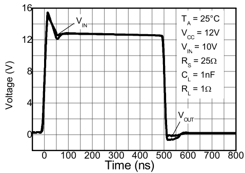
Switching Speed
