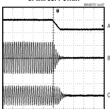
DPWM SOFT-START
