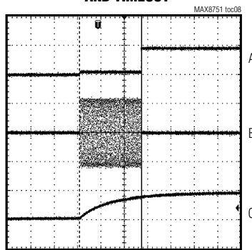
LAMP-OUT VOLTAGE LIMITING AND TIMEOUT
