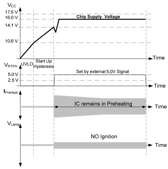
Figure 31 Start UP IC REMAINS in Pre Heating
