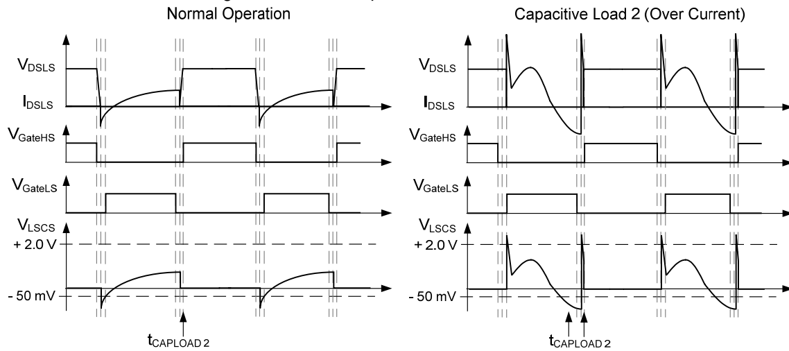
Figure 24 Capacitive Mode 2 – Operation with Over Current
