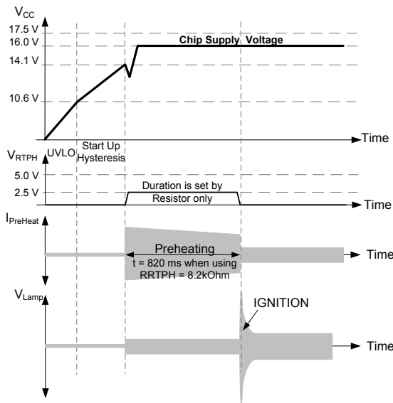
Figure 30 Start UP with Pre Heating
