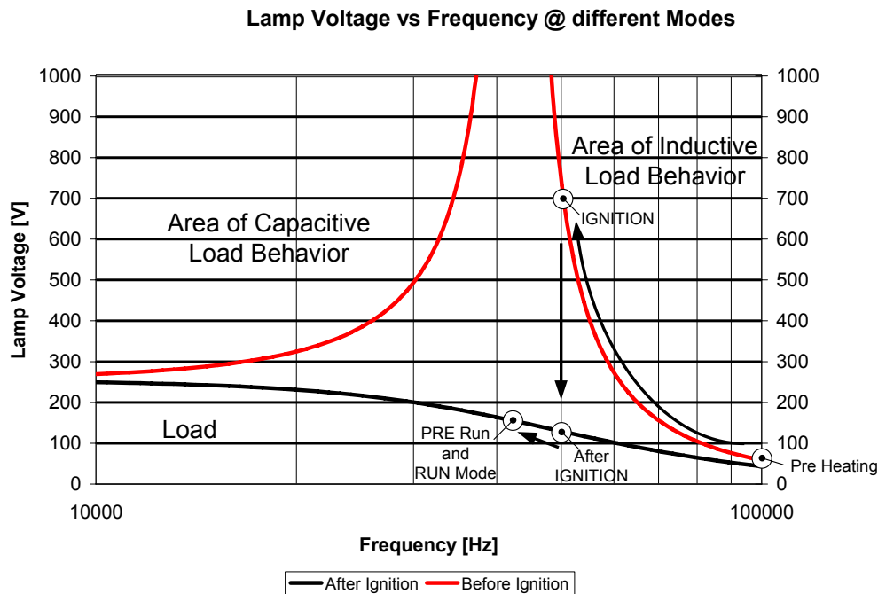
Figure 23 Capacitive and Inductive Operation
