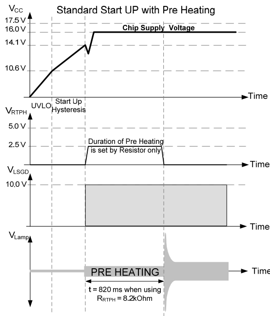
Figure 28 Start UP WITH Pre Heating
