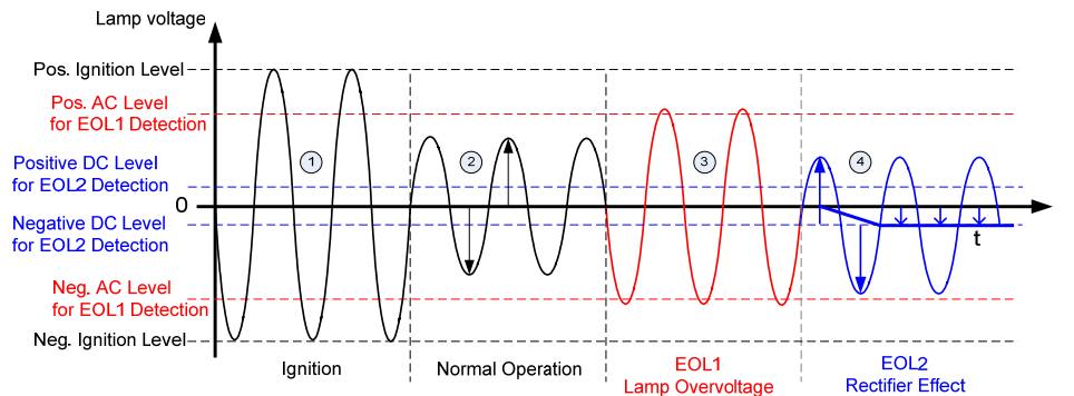
Figure 20 End of Life and Rectifier Effect
