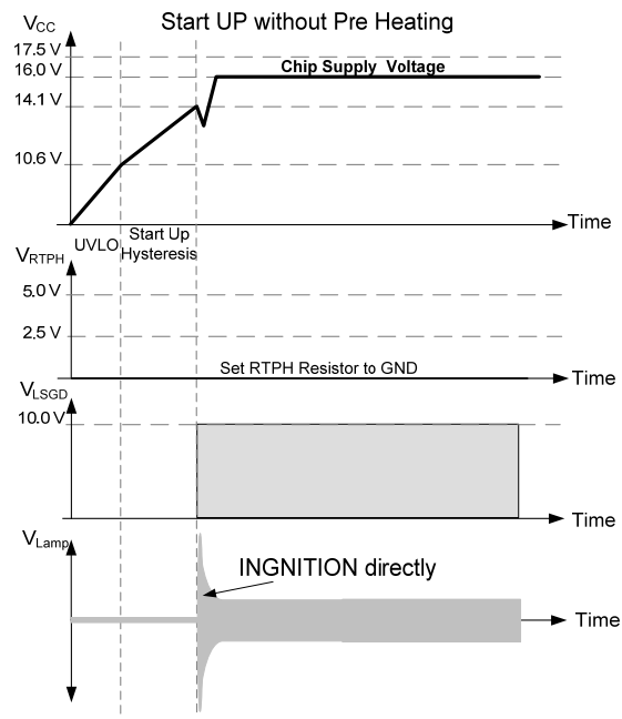
Figure 29 Start UP WITHOUT Pre Heating
