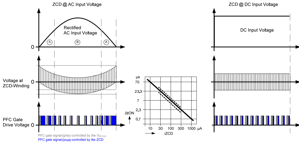
Figure 17 THD Optimization using adjustable Pulse Width Extension
