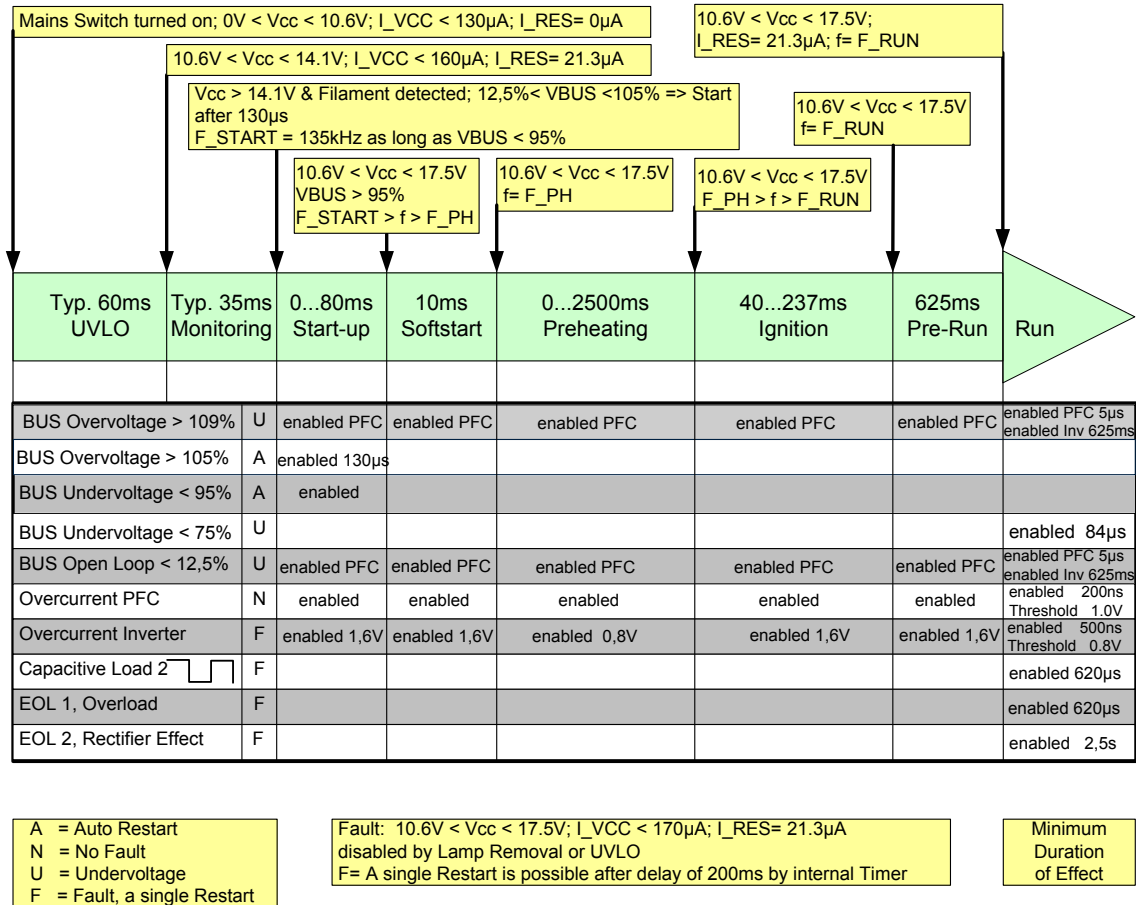
Figure 35 Monitoring Features during different operating Modes
