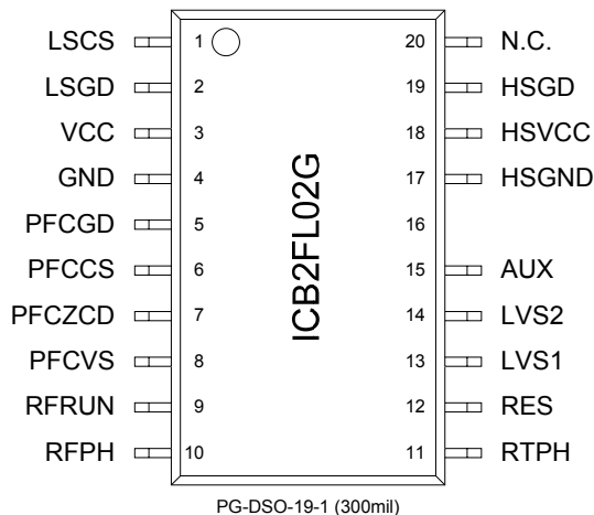
Figure 2 Package PG-DSO-19-1
