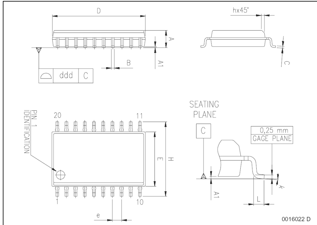
Figure 7. Package dimensions
