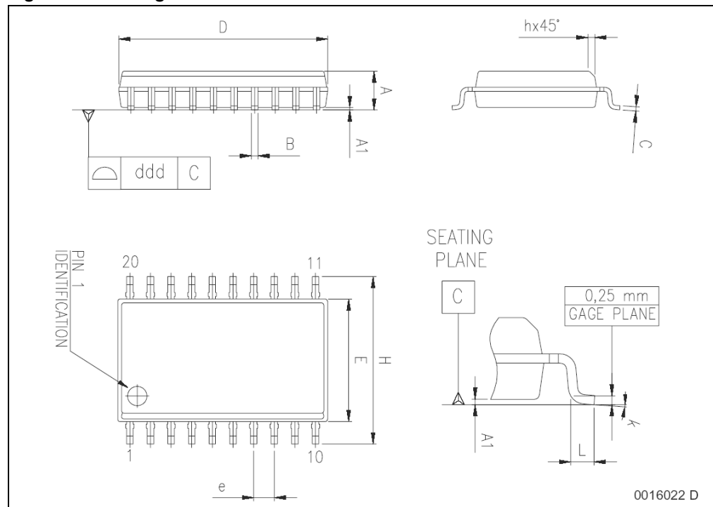
Figure 13. Package dimensions
