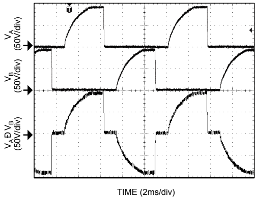
Figure 5. Typical 100Hz EL Driver for 3in² Lamp
