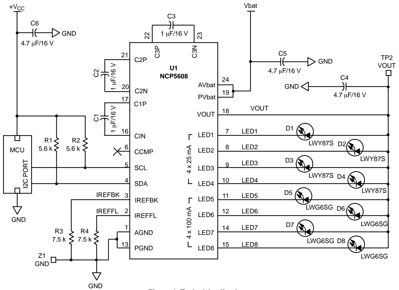
Figure 1. Typical Application
