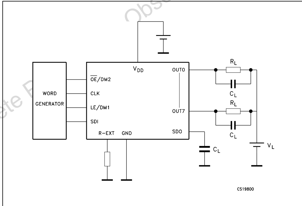
Figure 12. AC characteristics
