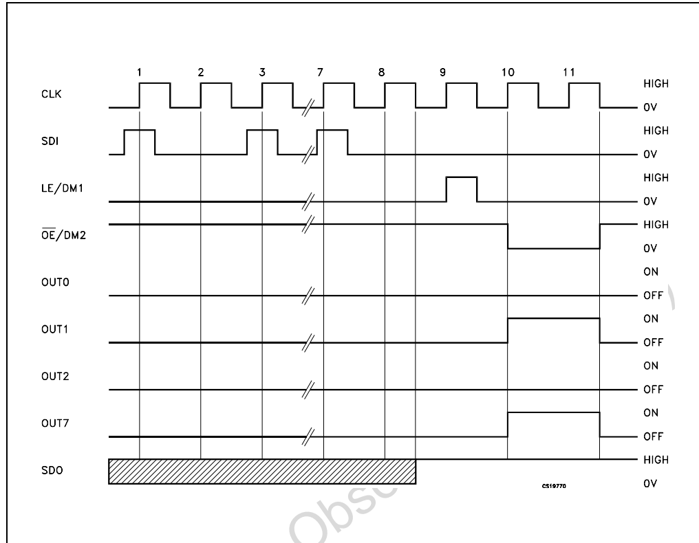
Figure 7. Timing diagram
