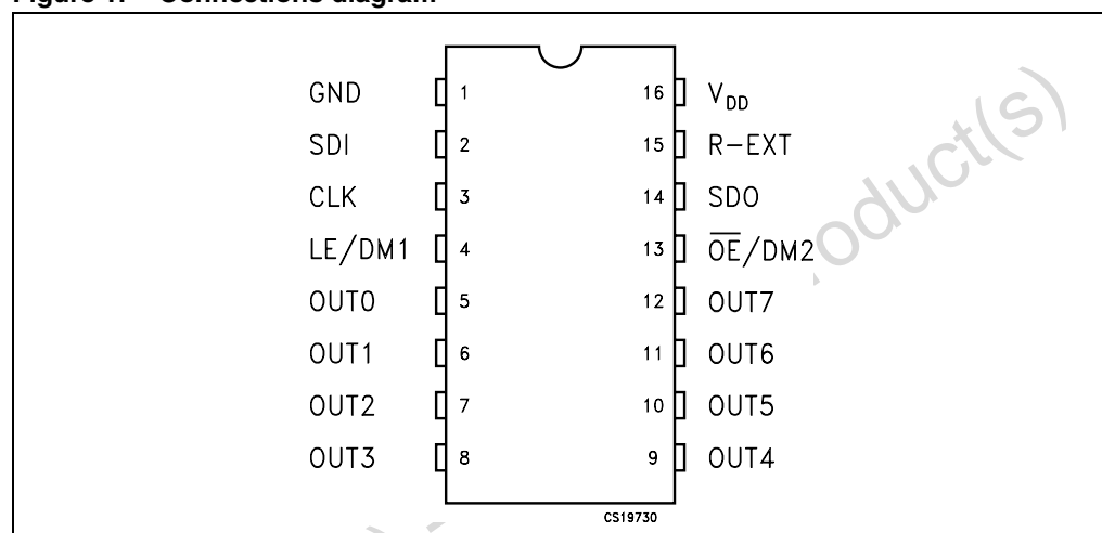
Figure 1. Connections diagram
