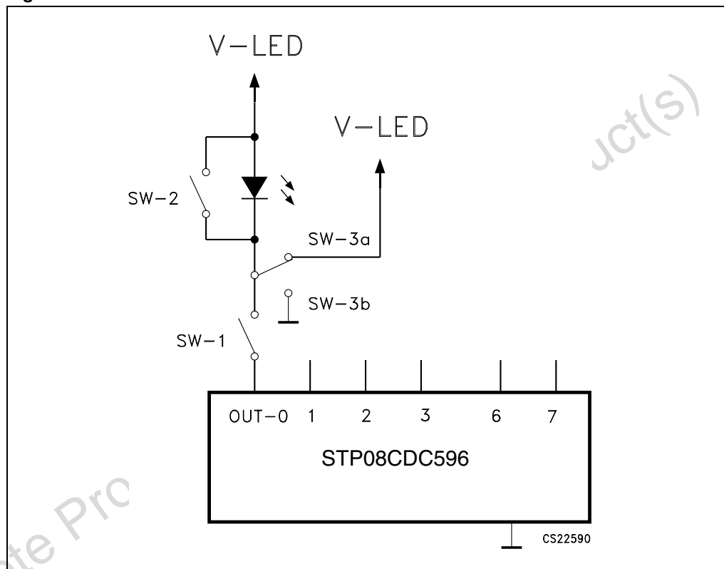
Figure 14. Detection circuit
