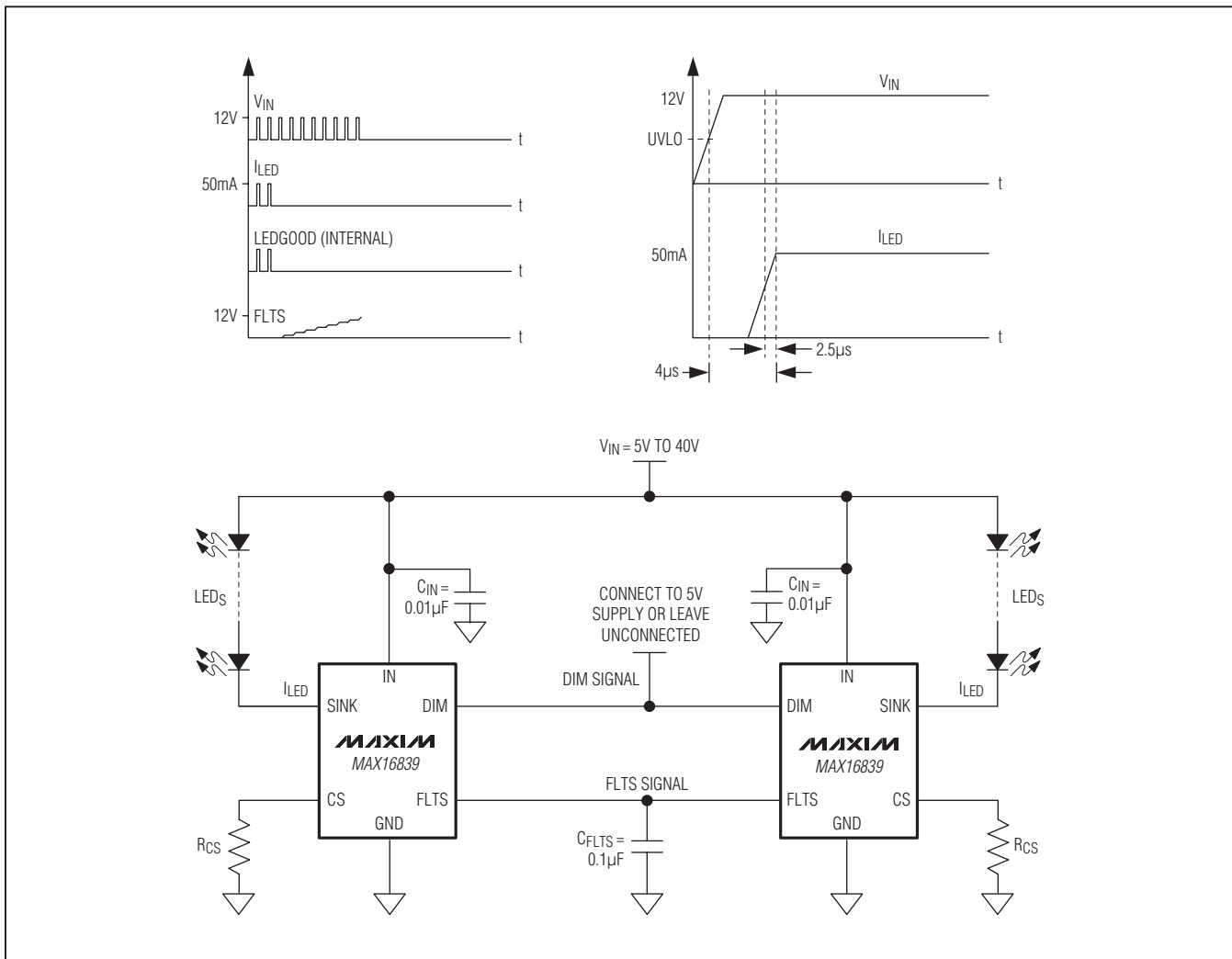
Figure 2. Multistring Application
