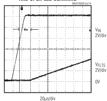
FAULT ACTIVATION THRESHOLD AND OPEN-LED BLANKING
