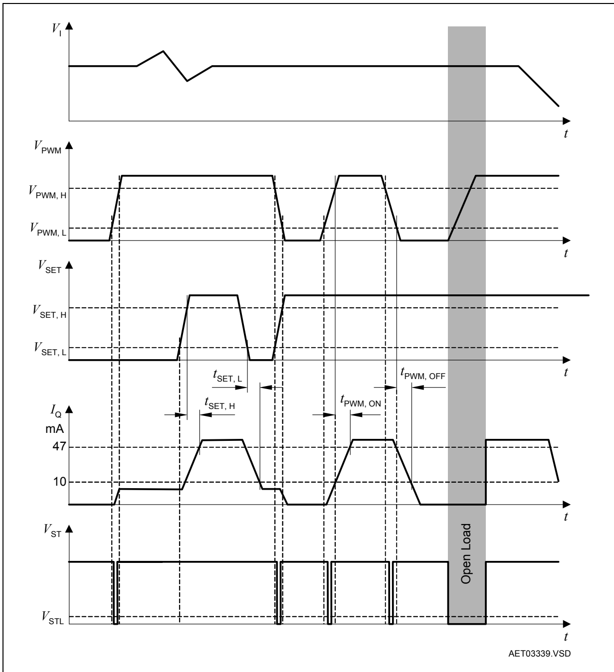
Figure 4 Function and Timing Diagram
