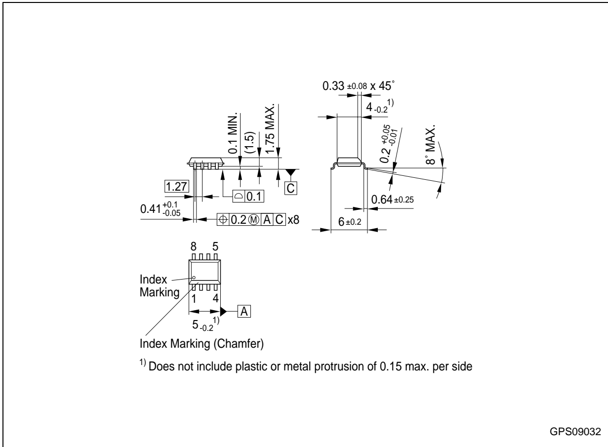
Figure 5 P-DSO-8-9 (Plastic Dual Small Outline)
