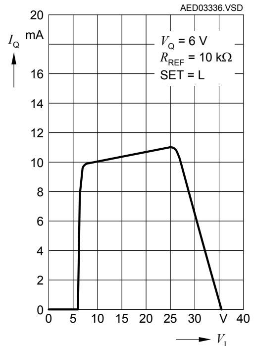
Output Current versus Supply Voltage, SET = L
