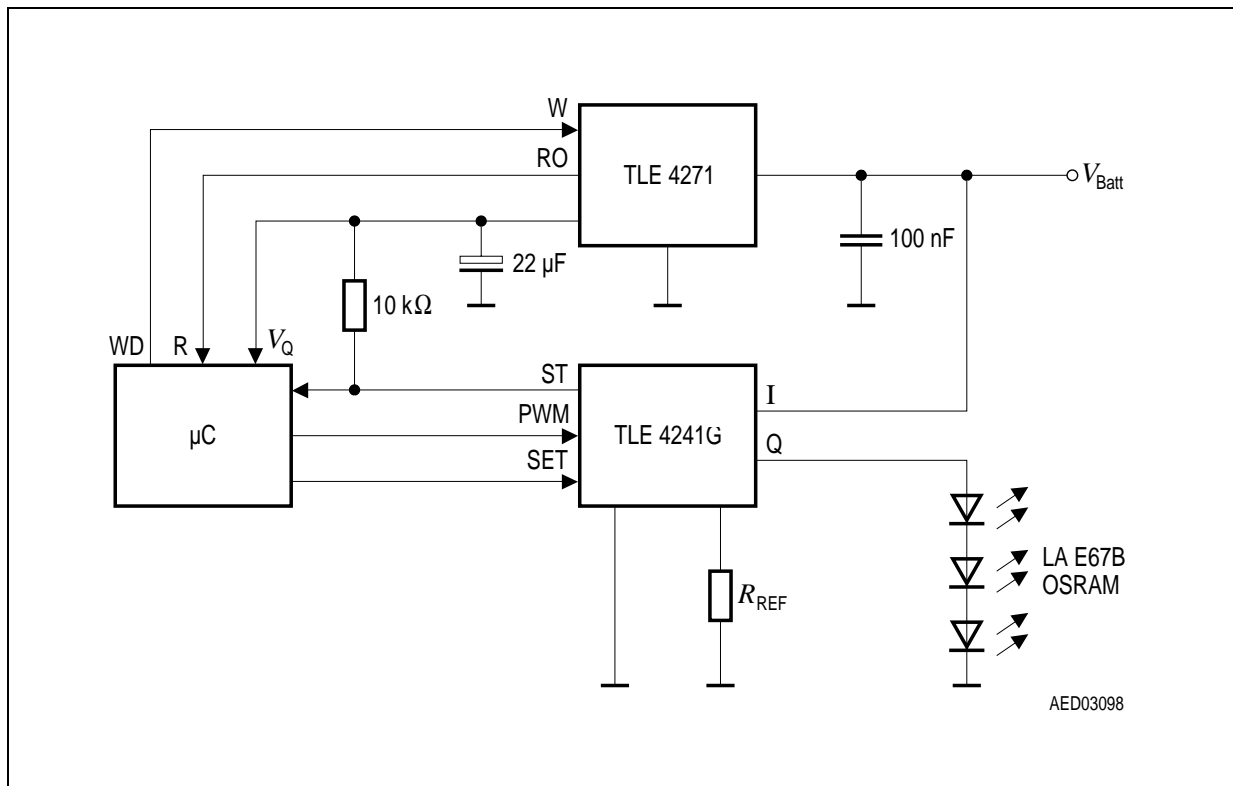
Figure 3 Application Circuit
