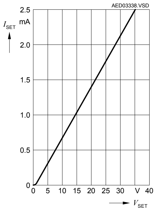
SET Pin Input Current versus SET Voltage
