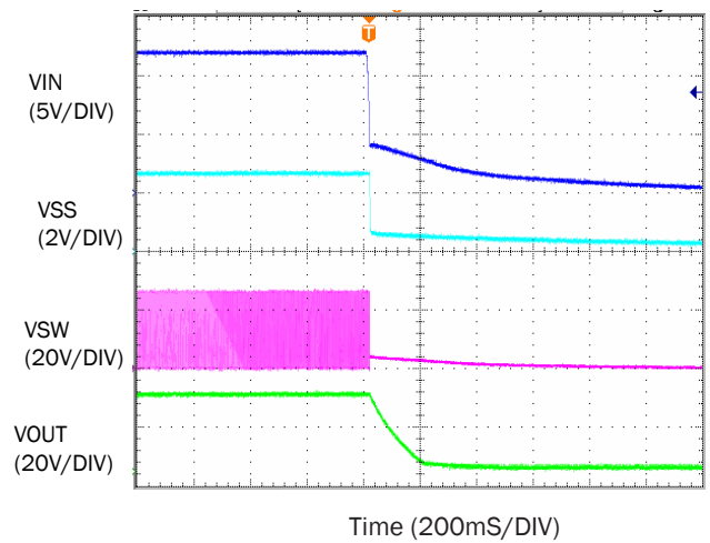
Conditions: VIN = 12V, Output = 27V / 20mA x 4 LED strings
