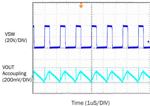
Conditions: VIN = 12V, Output = 36V / 150mA x 4 LED strings
