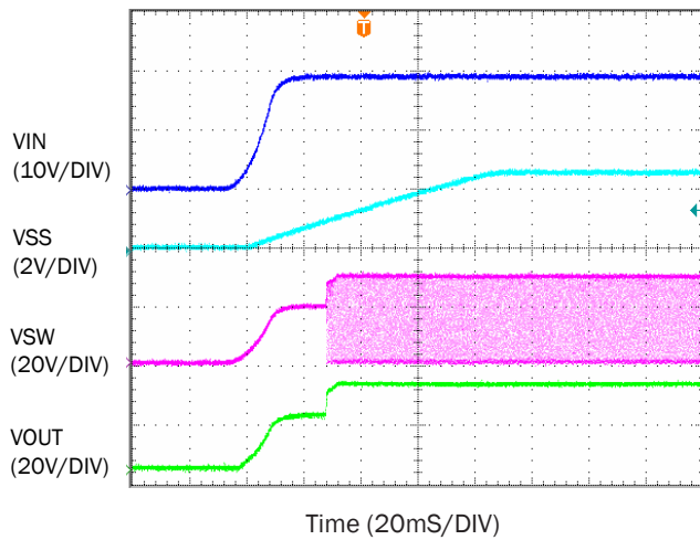
Conditions: VIN = 19V, Output = 30V / 150mA x 4 LED strings
