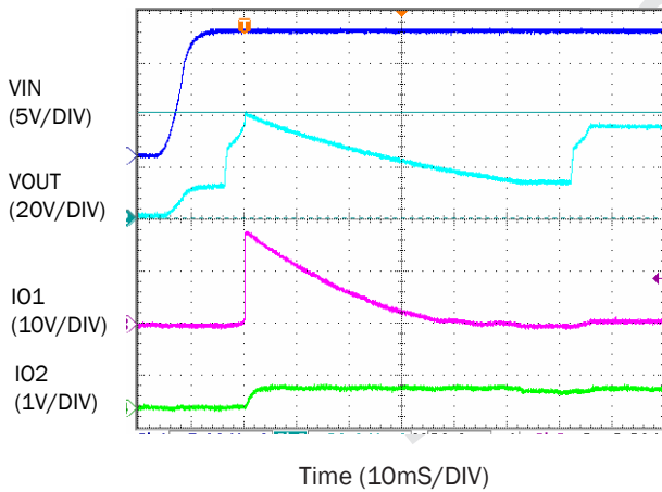
Conditions: VIN = 12V, I02 LED String is open circuit, Output = 36V / 150mA x 3 LED strings
