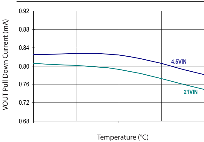
VOUT Pull Down Current vs. Temperature
