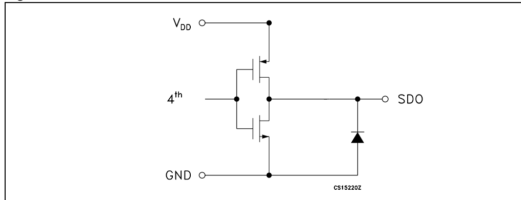
Figure 6. SDO terminal
