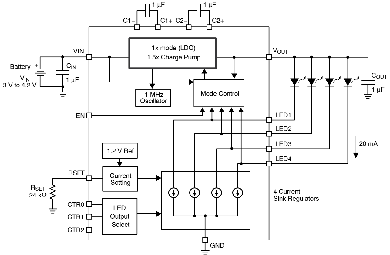
Figure 2. CAT3604 Functional Block Diagram
