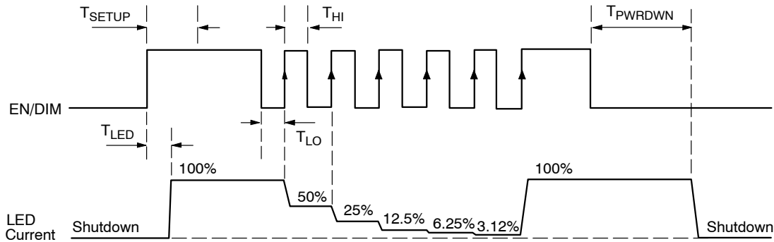
Figure 2. EN/DIM Dimming Timing Diagram
