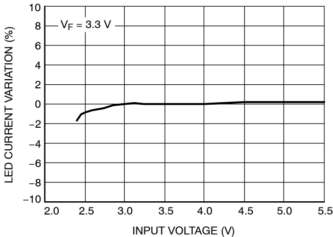
Figure 7. LED Current Change vs. Input Voltage
