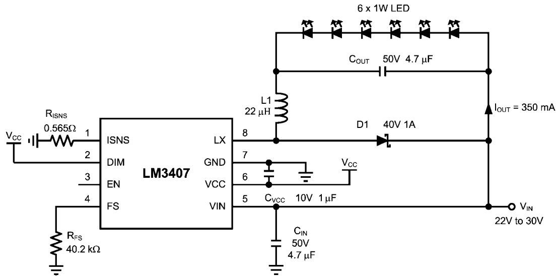
FIGURE 7. Typical Application Schematic for 6 LEDs
