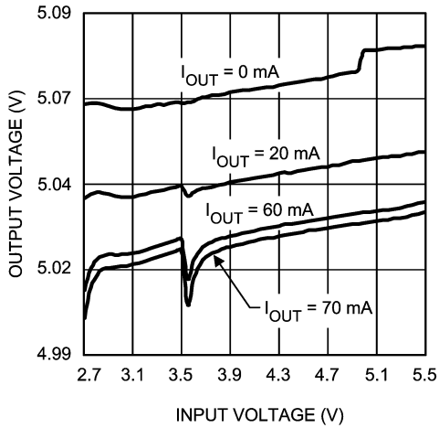
Output Voltage vs. Input Voltage, Version A (5V), 300kHz
