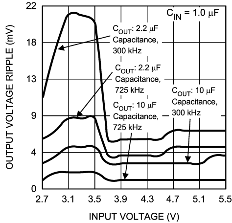
Output Voltage Ripple vs. Input Voltage Version B (4.5V), Load = 120mA
