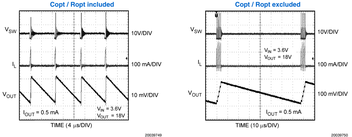
FIGURE 4. Output Ripple Voltage
