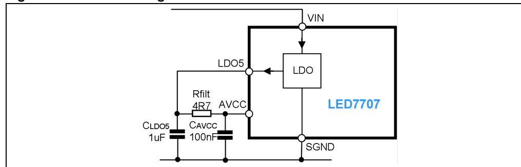
Figure 4. AVCC filtering
